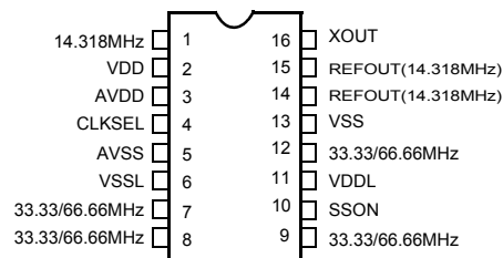
Figure 2. Table 3 Configuration Pinout
