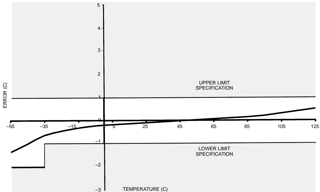
DS1821 TEMPERATURE READING ERROR
