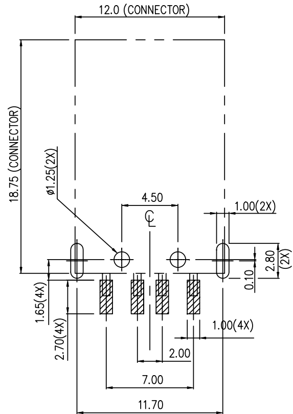
RECOMMENDED P.C.B. LAYOUT TOLERANCE: ±0.05
