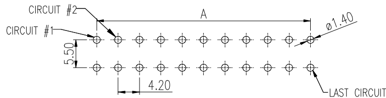
PCB LAYOUT COMPONENT SIDE
