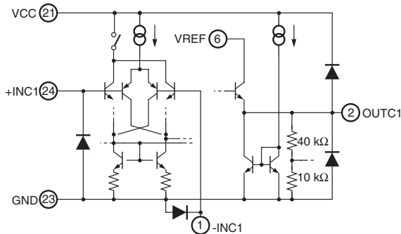
<Current detection amplifier block (Current Amp1) >
