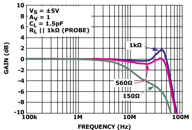
FIGURE 2. FREQUENCY RESPONSE FOR VARIOUS R_L
