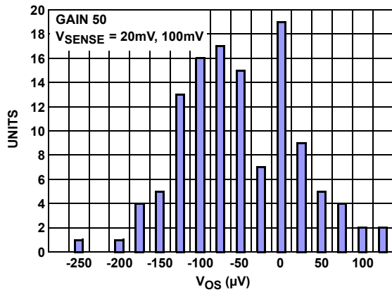
FIGURE 23. V_{OS} (µV) DISTRIBUTION AT +25°C, V_{RS+} = 12V , QUANTITY: 100
