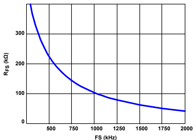
FIGURE 59. R_{FS} SELECTION vs F_S
