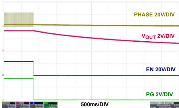
FIGURE 34. SHUTDOWN IN NO LOAD, PFM
