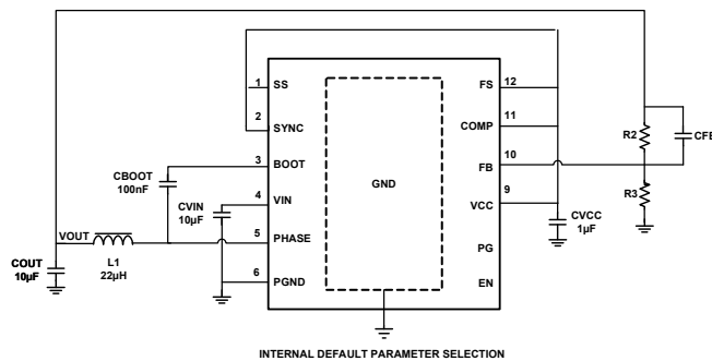
FIGURE 1. TYPICAL APPLICATION
