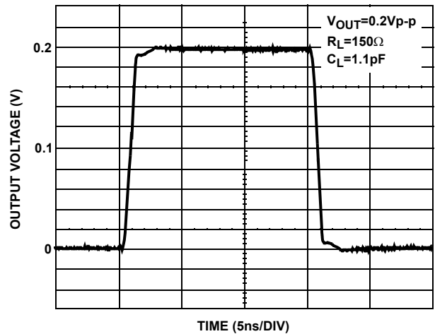
FIGURE 12. SMALL SIGNAL TRANSIENT RESPONSE; R_L=150\Omega
