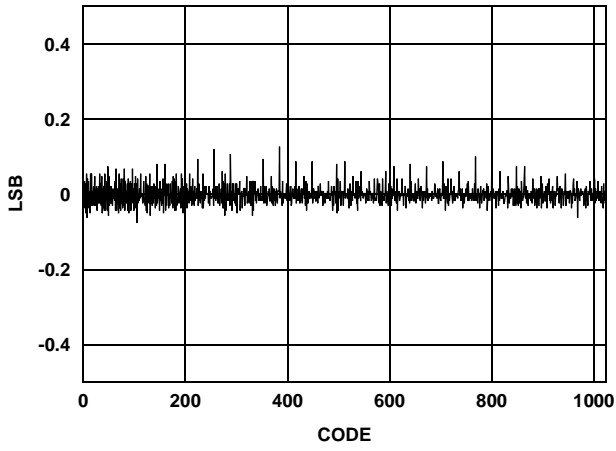
FIGURE 36. DIFFERENTIAL NONLINEARITY
