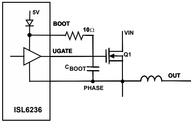
FIGURE 75. REDUCING THE SWITCHING-NODE RISE TIME
