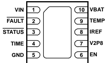
ISL9205D (10 LD DFN) TOP VIEW
