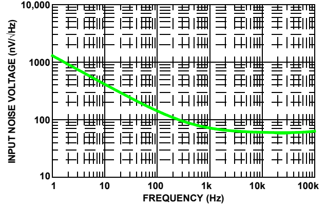
FIGURE 23. SIMULATED INPUT NOISE VOLTAGE
