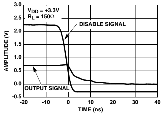
FIGURE 14. DISABLE TIME
