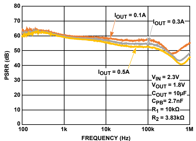
FIGURE 2. PSRR
