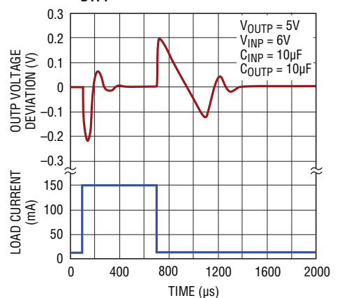
OUTP Transient Response C_BYPP = 0
