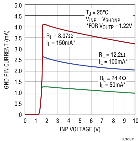
LT3032 Positive Side GND Pin Current
