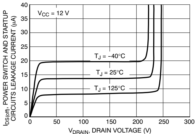
Figure 23. Power Switch Circuit and Startup Circuit Leakage Current vs. Drain Voltage
