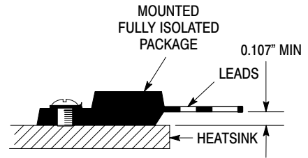
Figure 13. Screw Mounting Position for Isolation Test Number 3
