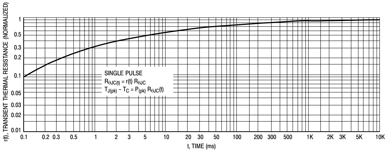
Figure 1. Thermal Response
