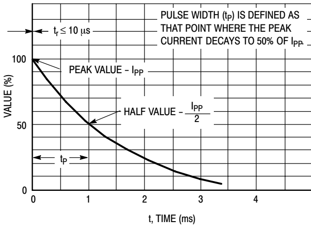
Figure 3. 10 \times 1000 \mu\text{s} Pulse Waveform
