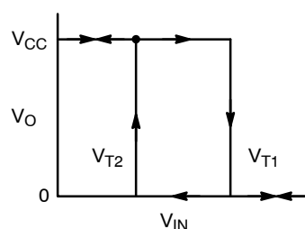
Figure 2. Hysteresis Curve
