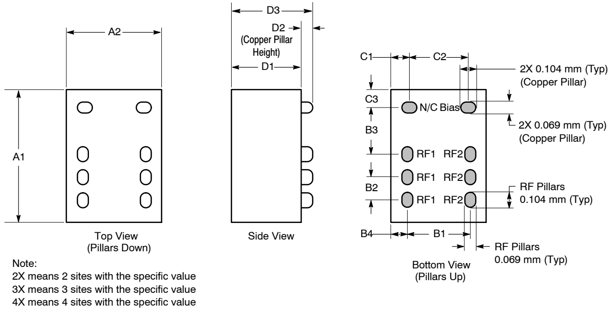
Figure 7. WLCSP Dimensions
