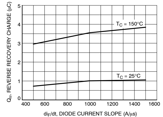
Figure 18. Stored Charge
