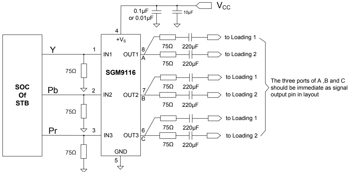
Figure 2. The DC Coupling Circuit Schematic is recommended in applications of STB
