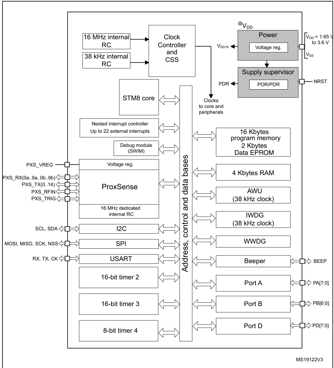
Figure 1. STM8TL5xx4 block diagram
