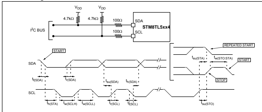
Figure 30. Typical application with I 2 C bus and timing diagram 1)
