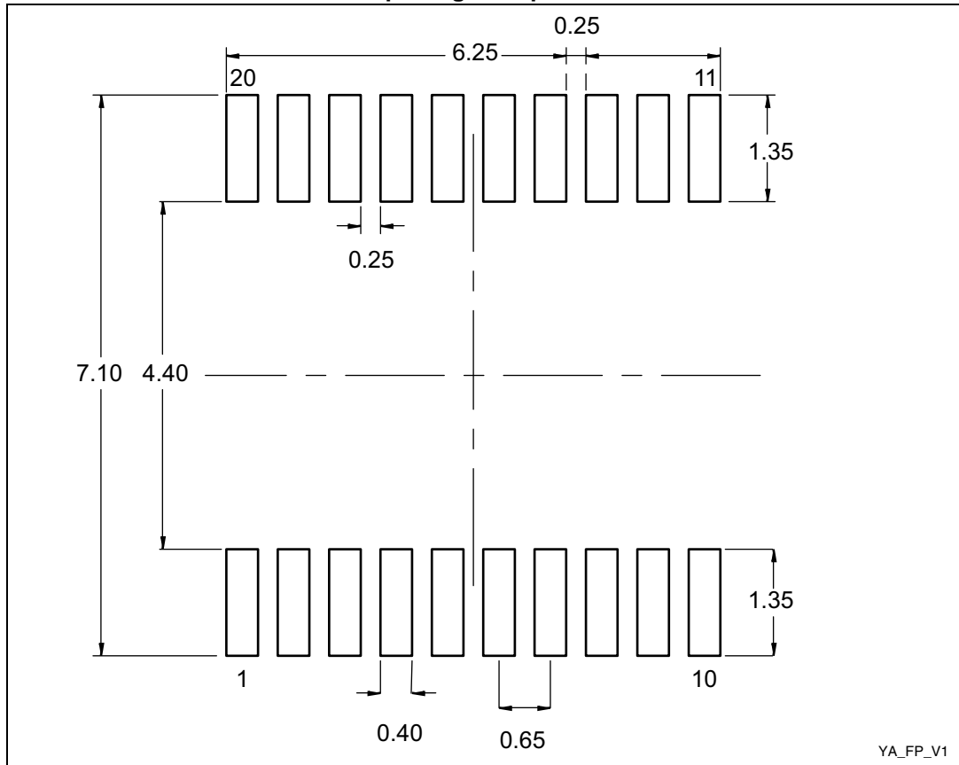
Figure 38. TSSOP20 – 20-lead thin shrink small outline, 6.5 x 4.4 mm, 0.65 mm pitch, package footprint
