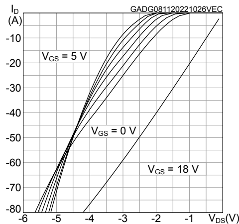
Figure 17. Typical reverse conduction characteristics ( T_J = 175^\circ\text{C} )
