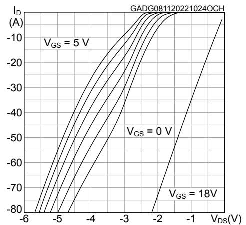
Figure 16. Typical reverse conduction characteristics ( T_J = 25^\circ\text{C} )
