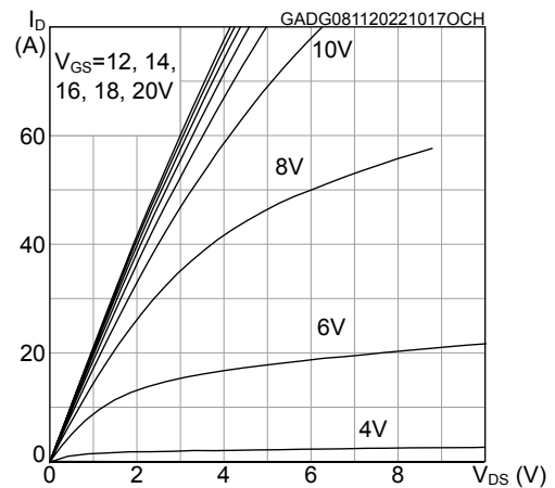
Figure 4. Typical output characteristics ( T_J = 175^\circ C )
