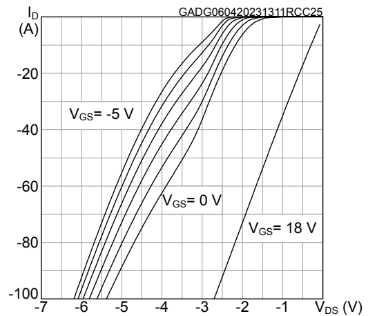
Figure 16. Typical reverse conduction characteristics ( T_J = 25 \text{ °C} )
