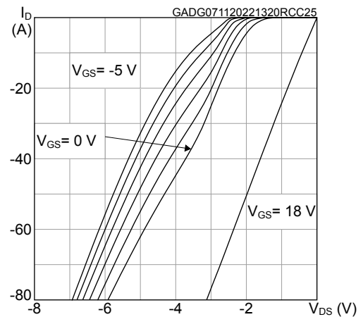
Figure 16. Typical reverse conduction characteristics ( T_J = 25 \text{ °C} )
