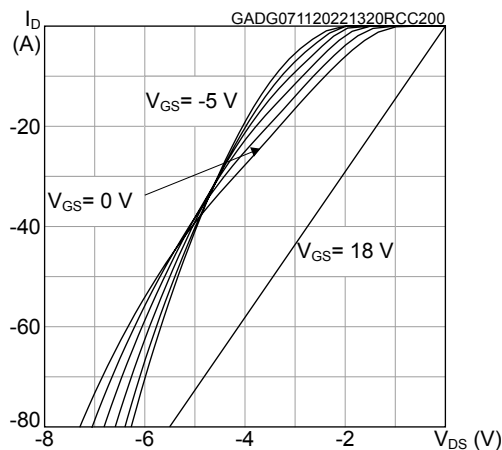
Figure 17. Typical reverse conduction characteristics ( T_J = 200 \text{ °C} )
