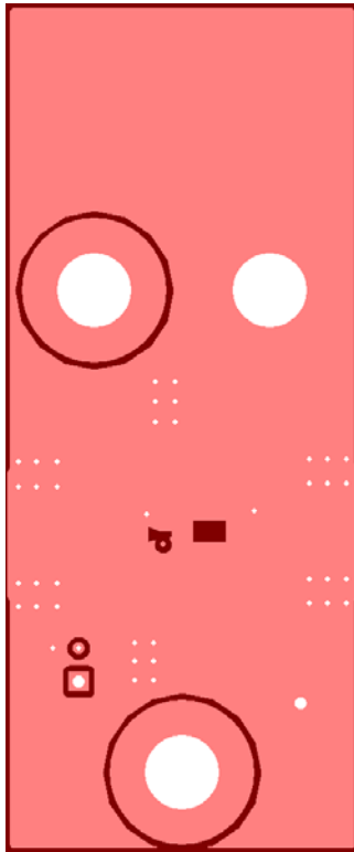
Figure 52. THS4302EVM Board Layout (Ground Layers 2 and 3)
