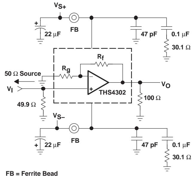
Figure 42. Wideband, Noninverting Gain Configuration
