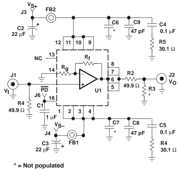
Figure 50. Typical THS4302 EVM Circuit Configuration
