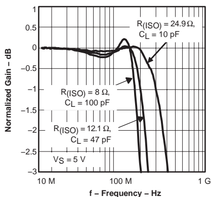
Figure 46. Driving Capacitive Loads
