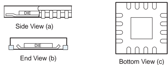
Figure 47. Views of Thermally Enhanced Package
