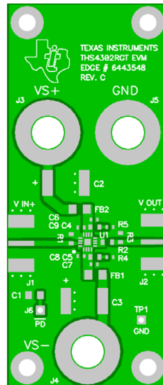
Figure 51. THS4302EVM Layout (Top Layer and Silkscreen Layer)
