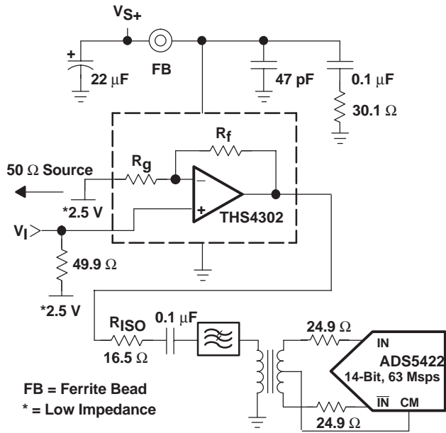
Figure 44. Driving an ADC Via a Transformer
