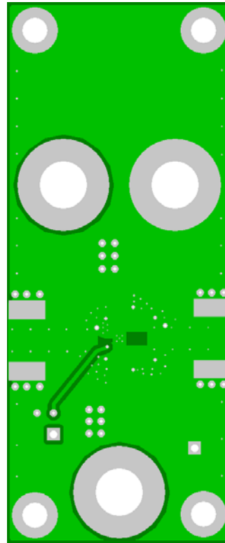
Figure 53. THS4302EVM Board Layout (Bottom Layer)
