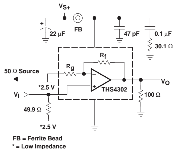
Figure 43. DC-Coupled Single Supply Operation
