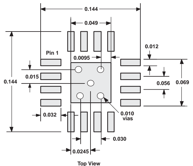
Figure 48. PowerPAD PCB Etch and Via Pattern
