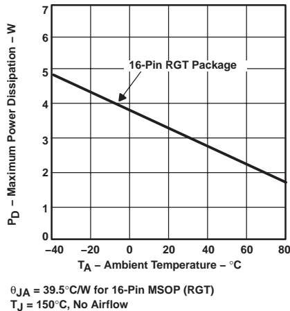
Figure 49. Maximum Power Dissipation vs Ambient Temperature
