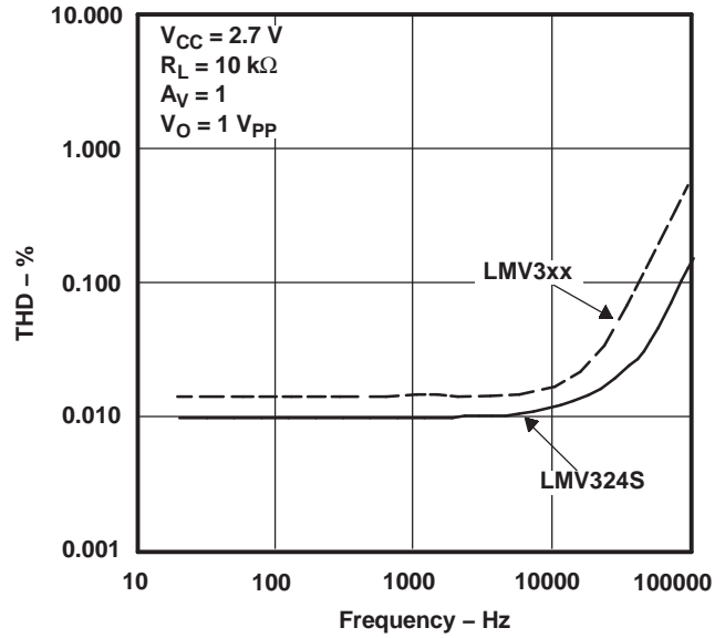
Figure 42. THD + N vs FREQUENCY
