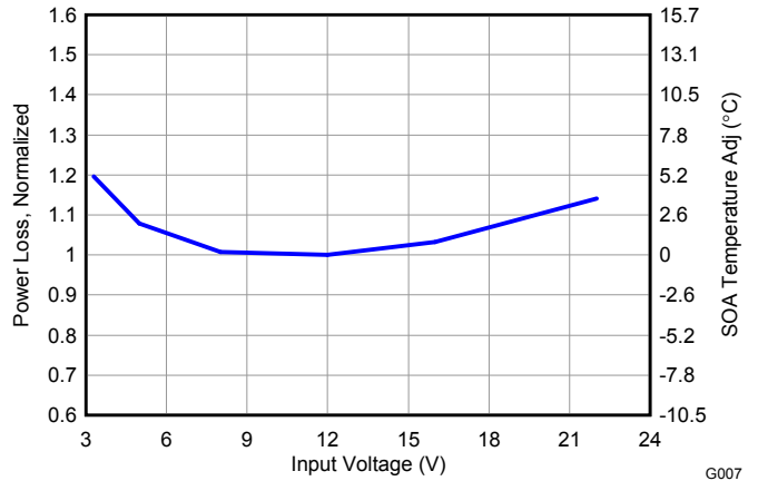
Figure 7. Normalized Power Loss vs Input Voltage
