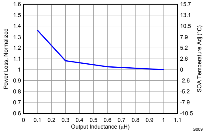
Figure 9. Normalized Power Loss vs. Output Inductance
