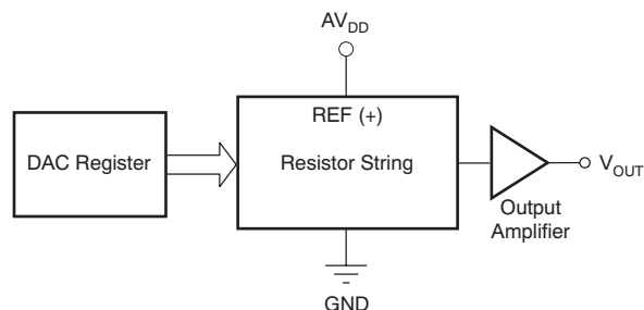
Figure 74. DAC8x11 Architecture
