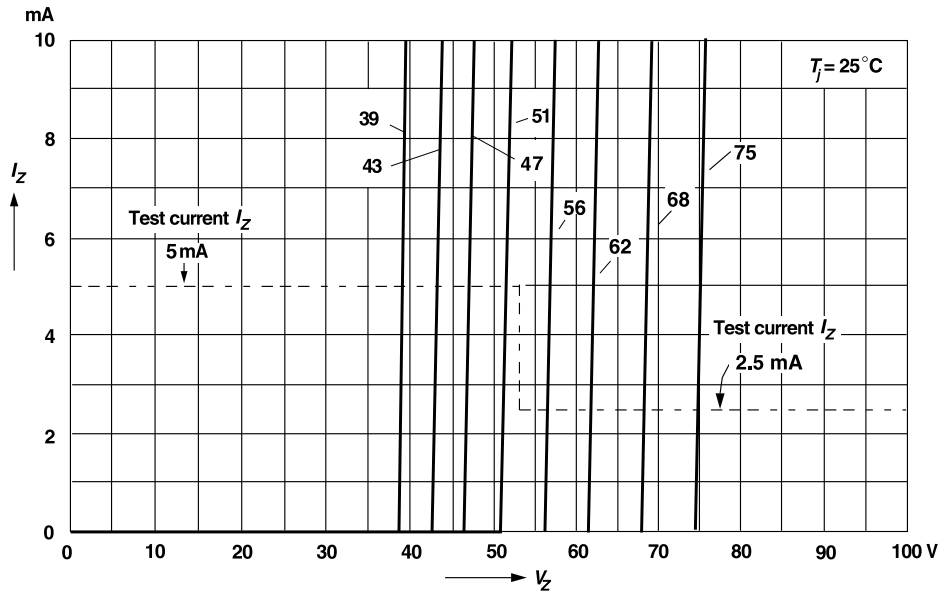
Figure 18. Breakdown Characteristics
