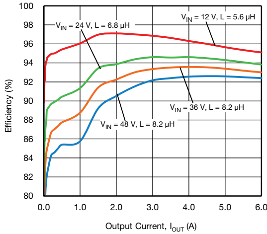
Fig. 17 - SiC462 Efficiency vs. Output Current, VOUT = 5 V
