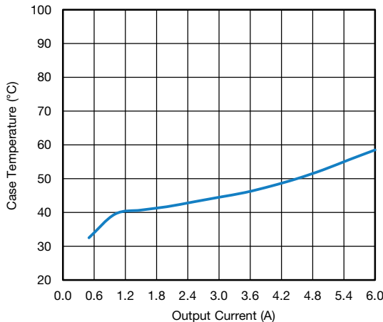
Fig. 19 - SiC462 Load Current vs. Case Temperature, VIN = 48 V, VOUT = 5 V
