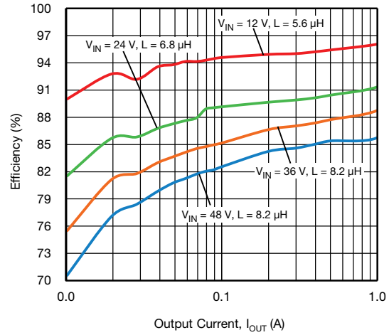
Fig. 20 - SiC462 Efficiency vs. Output Current - Light Load, VOUT = 5 V
