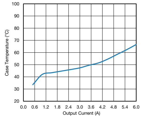
Fig. 22 - SiC462 Load Current vs. Case Temperature, VIN = 48 V, VOUT = 12 V
