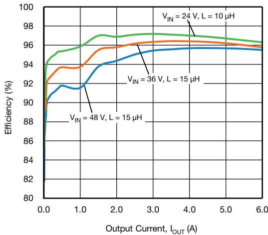
Fig. 18 - SiC462 Efficiency vs. Output Current, VOUT = 12 V
