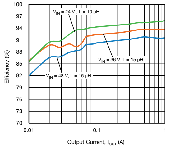
Fig. 21 - SiC462 Efficiency vs. Output Current - Light Load, VOUT = 12 V
