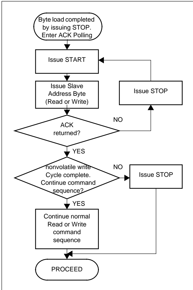
Figure 10. Acknowledge Polling Sequence
