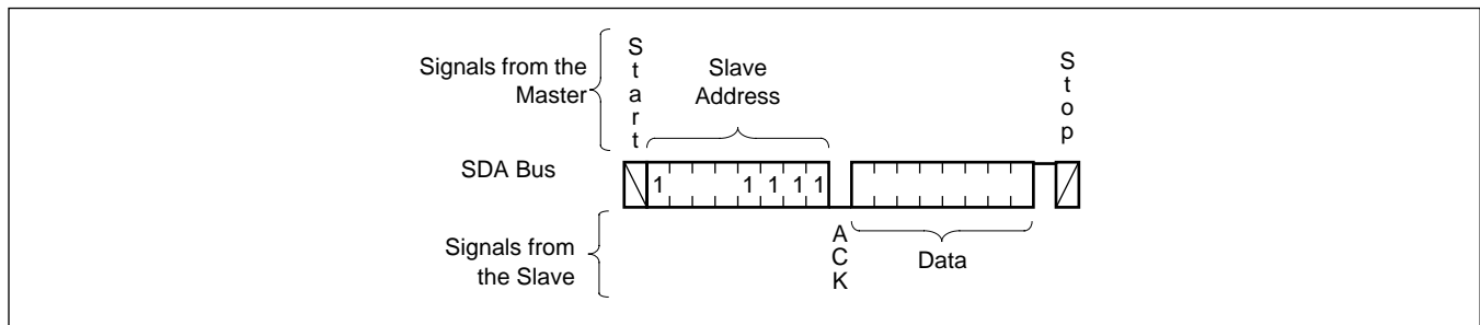
Figure 9. Current Address Read Sequence
