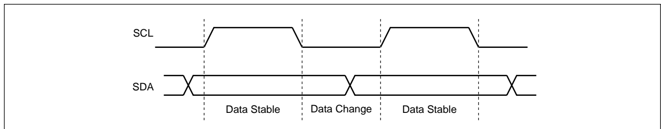
Figure 3. Valid Data Changes on the SDA Bus
