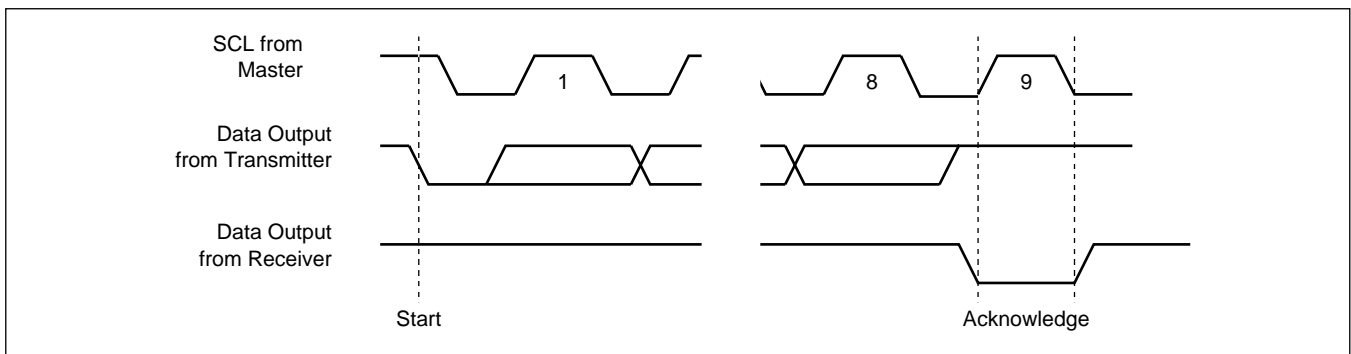
Figure 5. Acknowledge Response From Receiver
