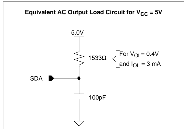
Figure 13. Standard Output Load for testing the device with V_{CC} = 5.0\text{V}
