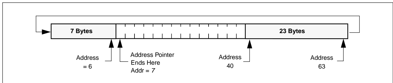
Figure 7. Writing 30 bytes to a 64-byte memory page starting at address 40.
