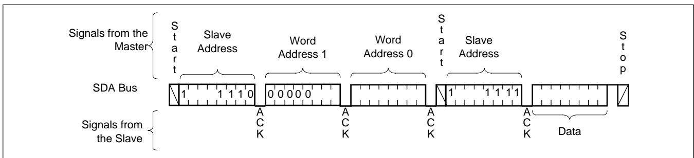
Figure 11. Random Address Read Sequence
