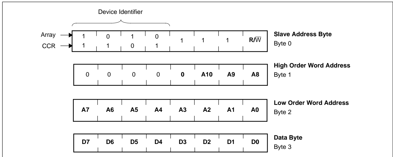
Figure 12. Slave Address, Word Address, and Data Bytes (64 Byte pages)
